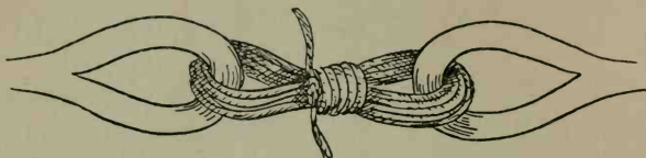
FIG. 97.—Rose lashing.
